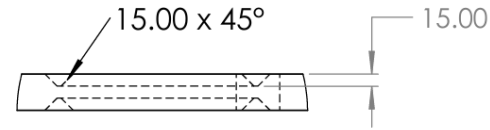
DETAIL A SCALE 1 : 8
